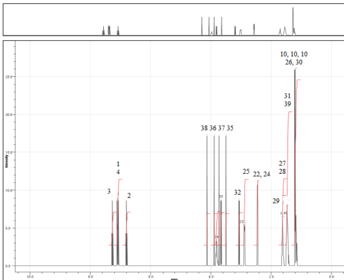
Figure 62: Better resolution of 1 H-NMR spectrum of (AZ-7) by Marvin Sketch.
